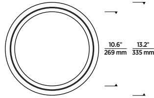
12" FLANGED
