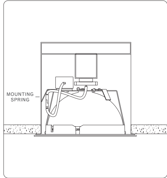
Installed fixture with fully engaged mounting springs.
