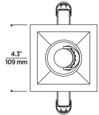
SHOWN IN SQUARE FLANGED AT NO TILT (0°)
