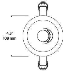
SHOWN IN ROUND FLANGED AT NO TILT (0°)
